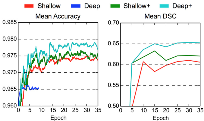
Fig. 7. Mean accuracy over validation samples and DSC for the segmentations of the validation images, as obtained from the “Shallow” baseline and “Deep” variant with smaller kernels. Training of the plain deeper model fails (cf. Section 3.3). This is overcome by adopting the initialization scheme of He et al. (2015), which further combined with Batch Normalization leads to the enhanced (+) variants. Deep+ performs significantly better than Shallow+ with similar computation time, thanks to the use of small kernels.
